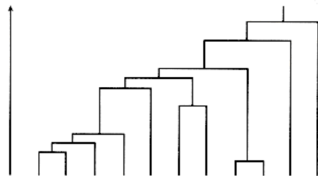
Figure 4.2: Dendrogram of a hierarchical classification
