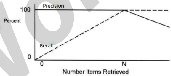
1.2a Ideal Precision and Recall
