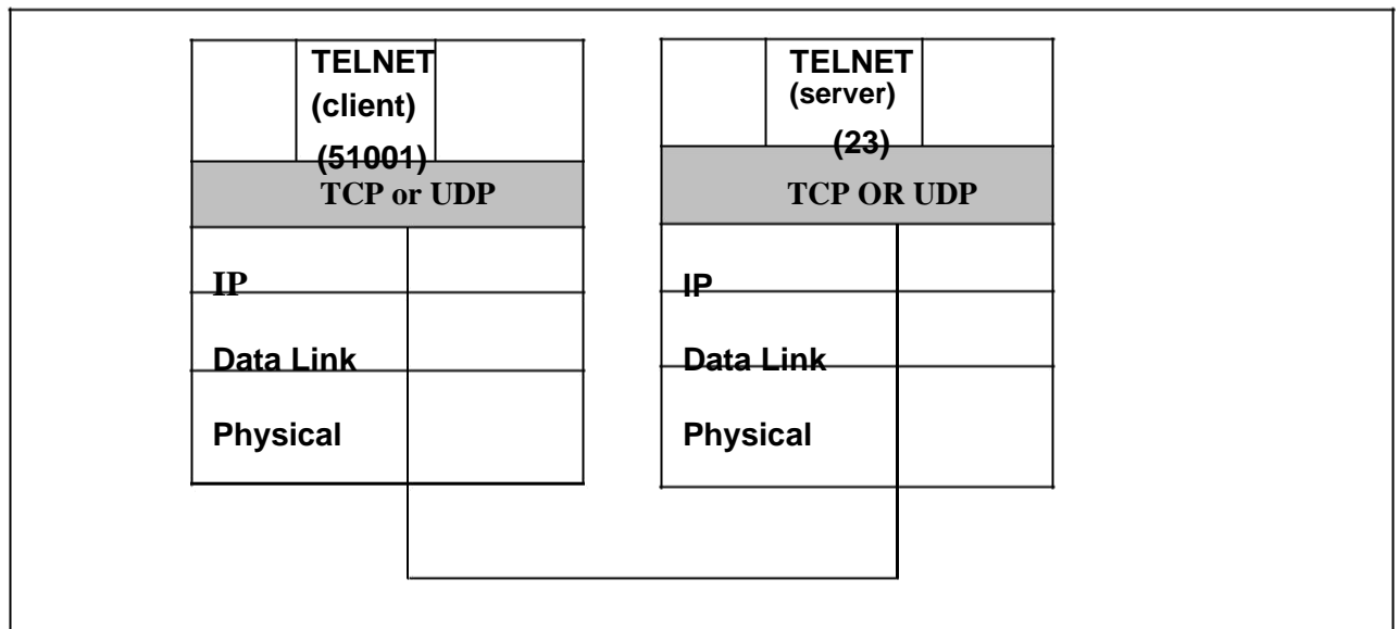
Figure Port addresses
