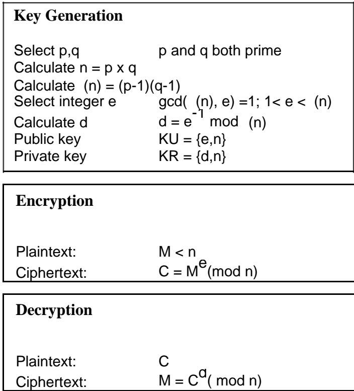
The RSA Algorithm (a)
