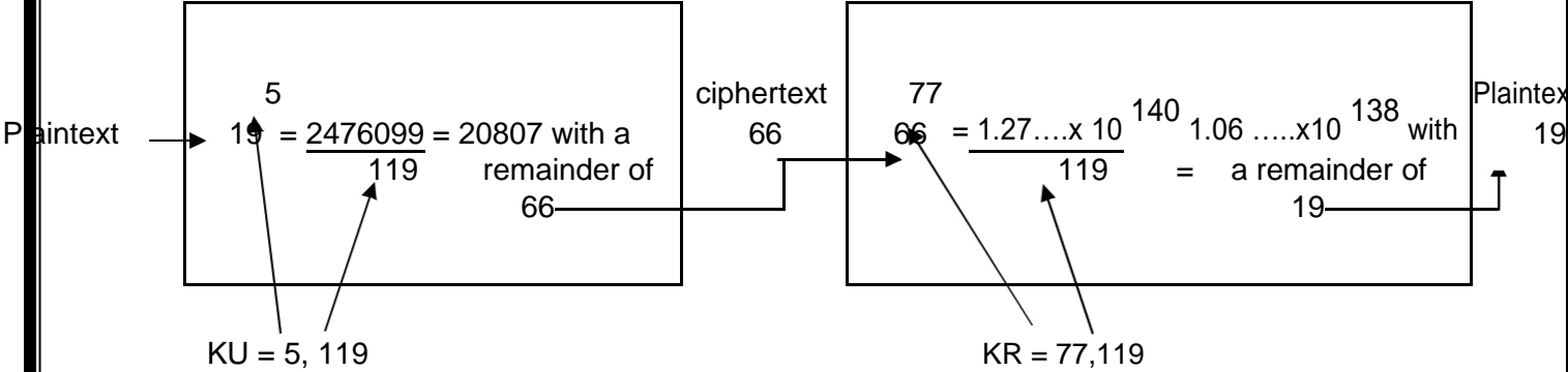
Example of RSA algorithm (b)
