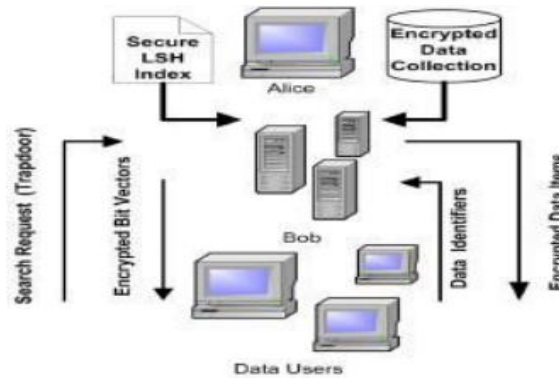
Fig. 1. Basic Secure Search Protocol
