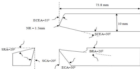
Fig. 3.1 Signature of the present cutting tool employed in solid modeling
