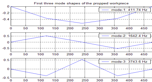
Fig.3.3 First three modes of propped cantilever work-piece
