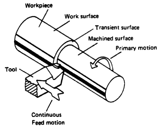
Figure 1.1 : Cylindrical turning on a lathe
