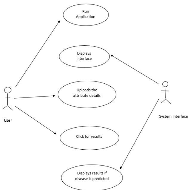
Fig. 2. Use-Case diagram
